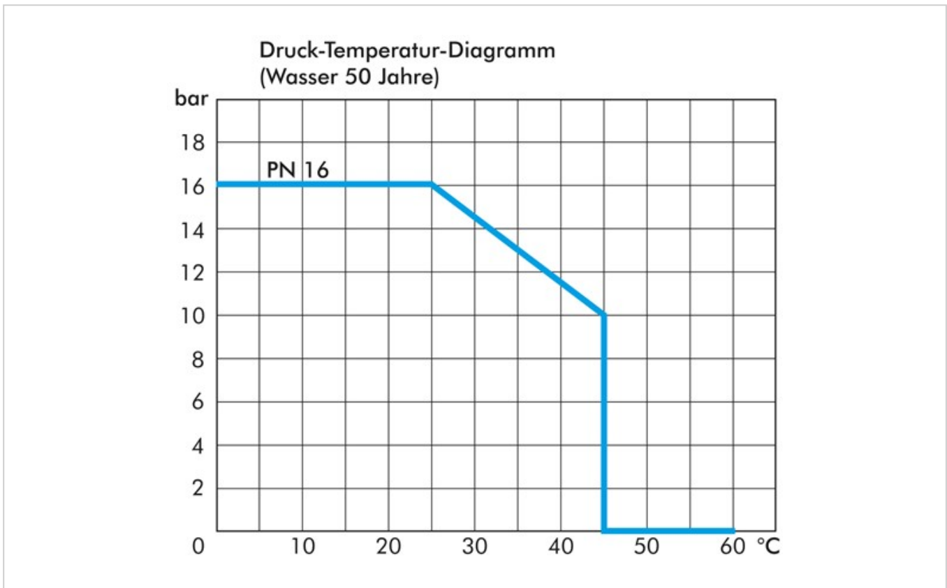
Drawing: Pressure-temperature diagram
