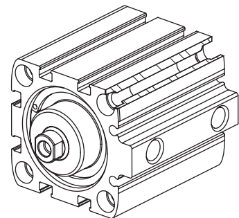
Ø 8 to 25 : 2 mounting holes per face Ø 32 to 100 : 4 mounting holes per face
