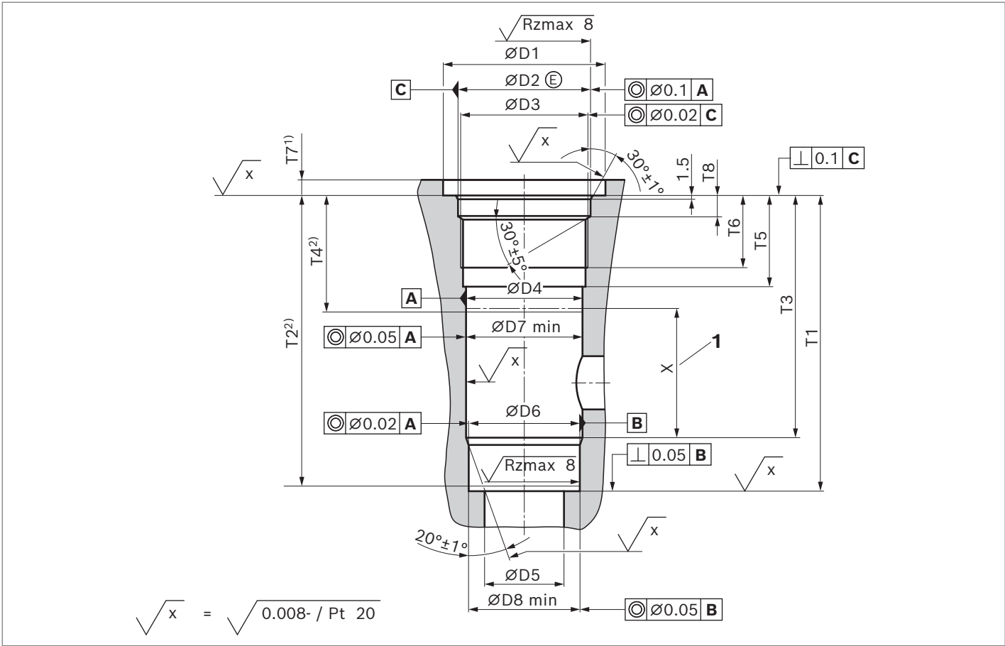
1 Area for outlet bore
