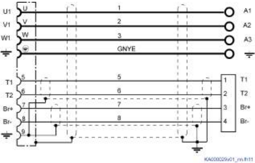
6.0 mm 2 wires 1, 2, 3, GNYE 1.0 mm 2 wires 5, 6 1.5 mm 2 wires 7, 8 Tab. 28-99: Interconnection diagram IKG4215
