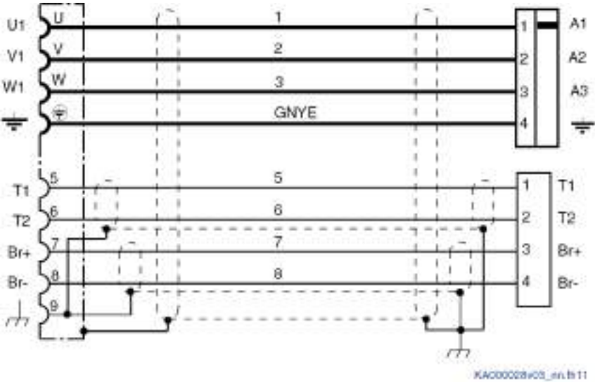
2.5 mm² wires 1, 2, 3, GNYE 1.0 mm² wires 5, 6, 7, 8 Tab. 28-145: Interconnection diagram RKL4308
