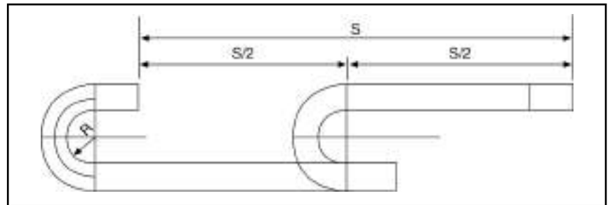
Fig. 6-4: Travel path
