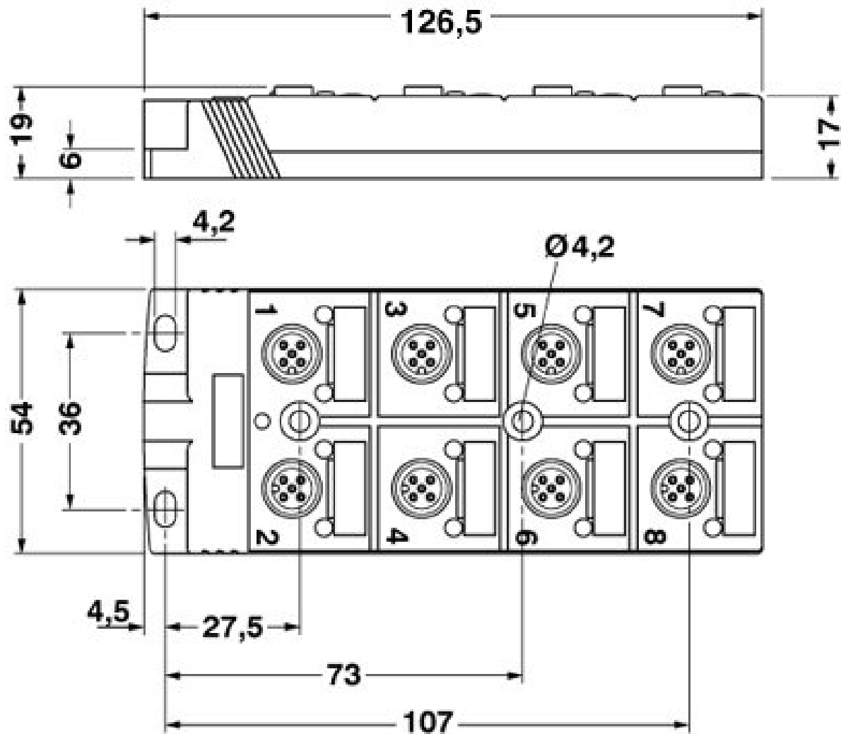
Dimensional drawing
