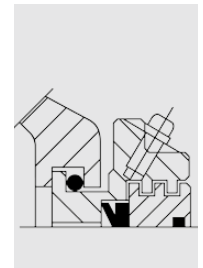
Joints de type TACK
