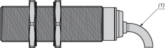
(1) Bending cable: 4 x external cable diameter
