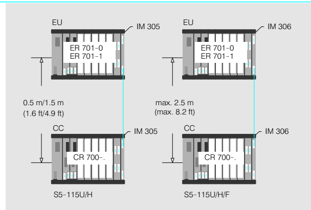
Fig. 3/2 Central connection of expansion units
