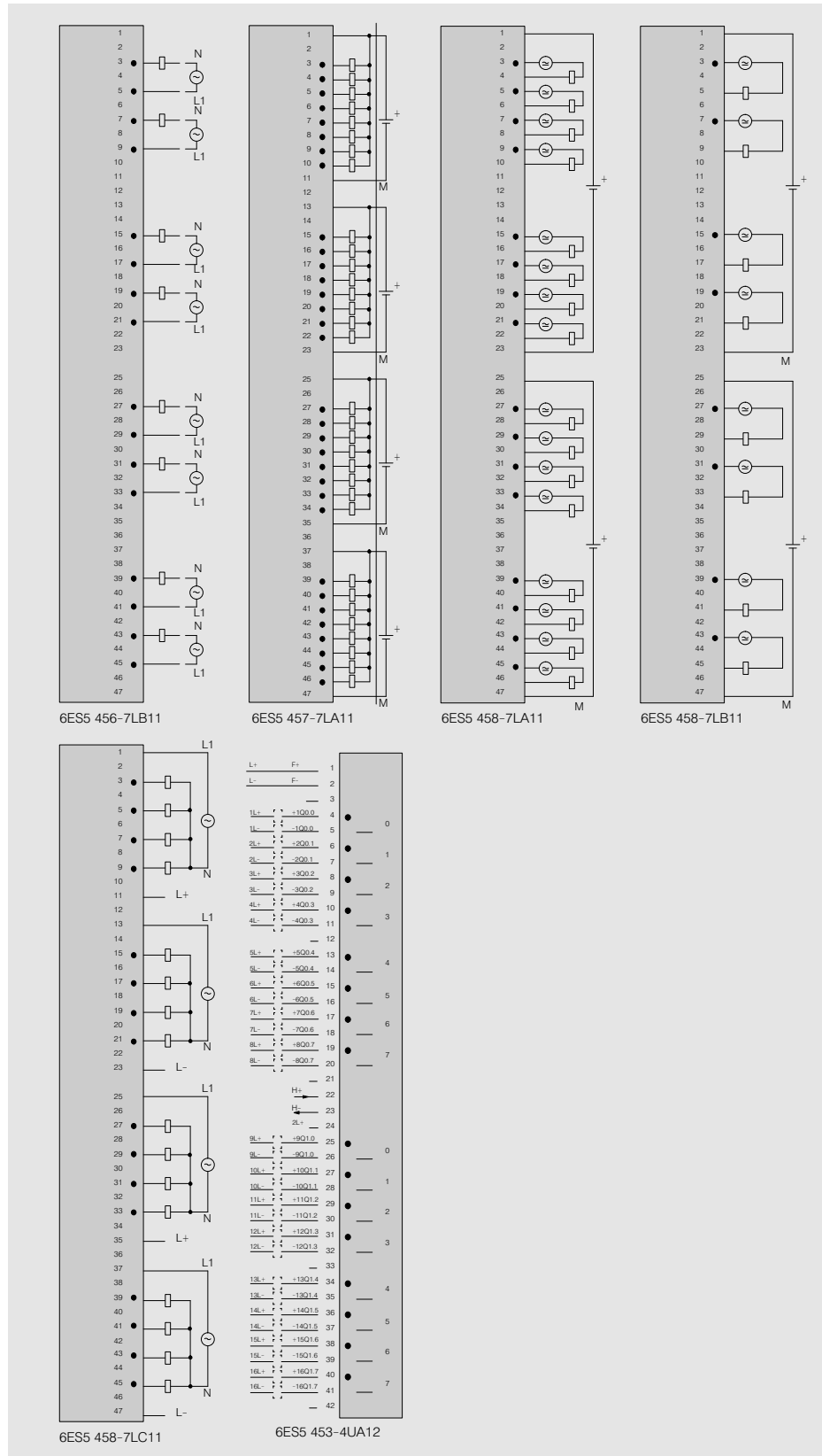
Fig. 3/28 Connection diagrams for digital output modules
