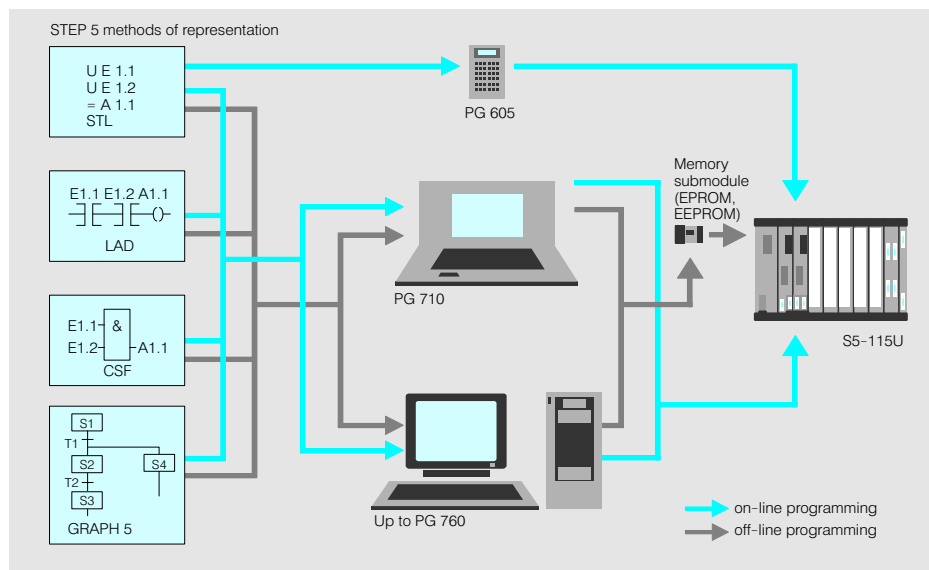
Fig. 3/5 Programming the S5-115U programmable controller
