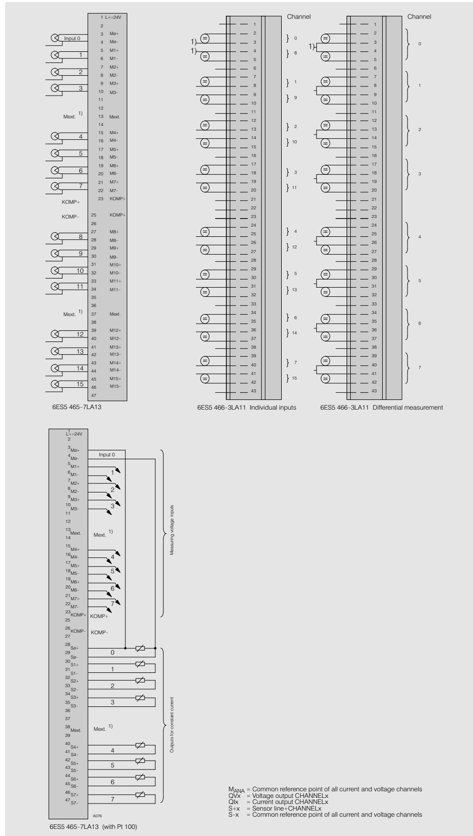
Fig. 3/31 Connection diagrams for analog input modules
