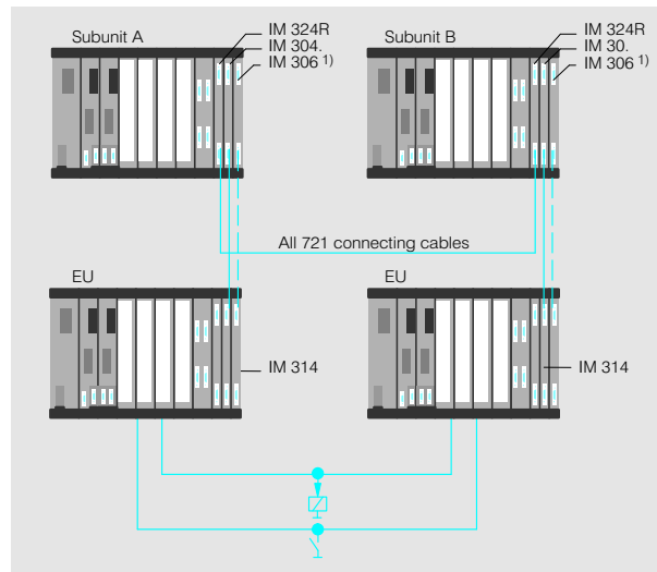
Fig. 3/11 Two-channel configuration (maximum fault tolerance)
