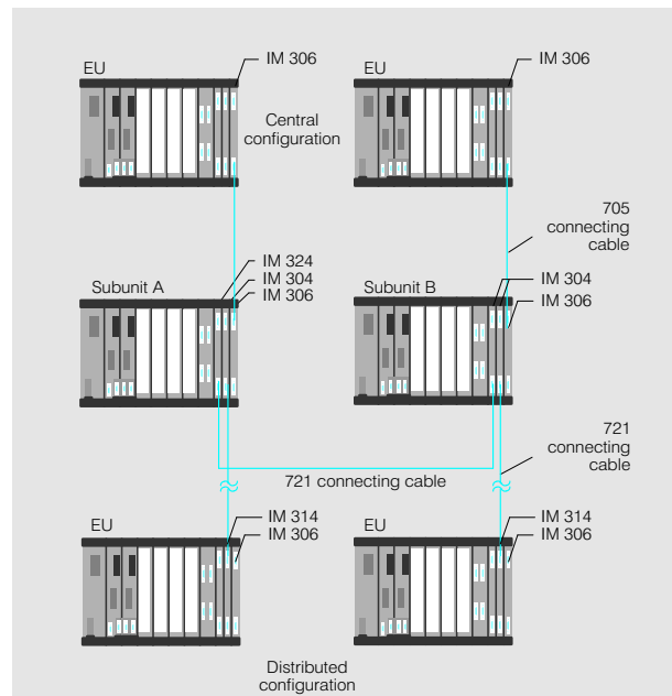
Fig. 3/18 Two-channel (redundant) I/O configuration (failsafe)
