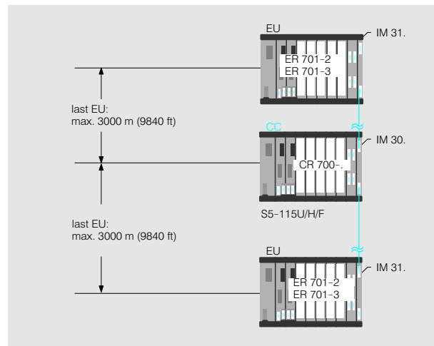
Fig. 3/3 Distributed connection of expansion units
