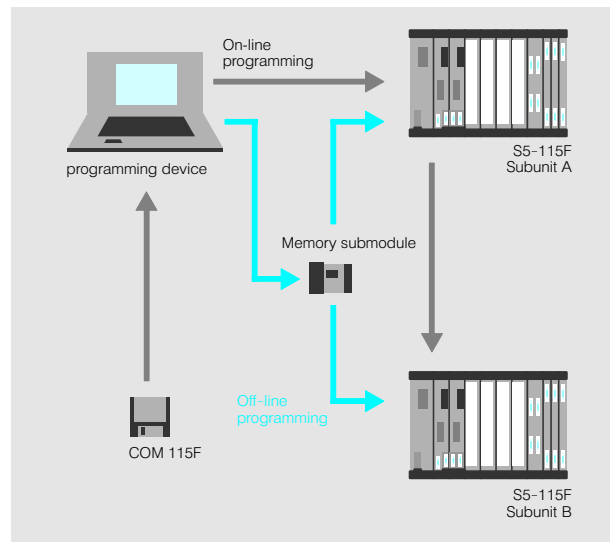
Fig. 3/21 On-line and off-line programming
