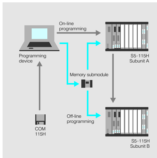
Fig. 3/15 On-line and off-line programming
