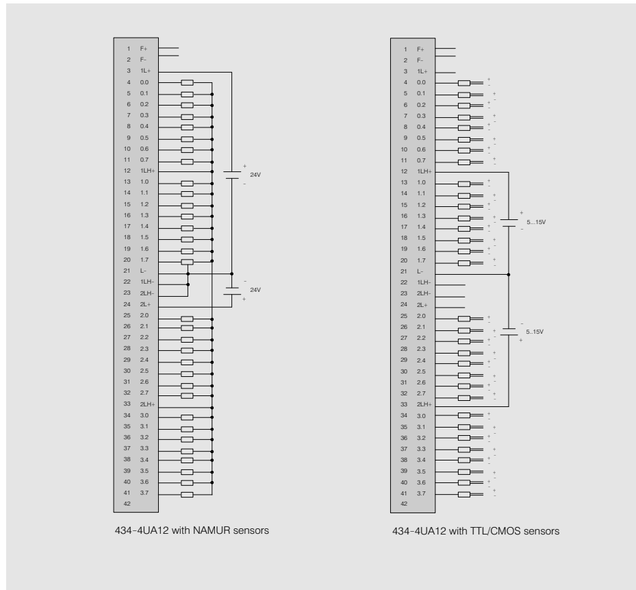
Fig. 3/26 Connection diagrams for digital input modules
