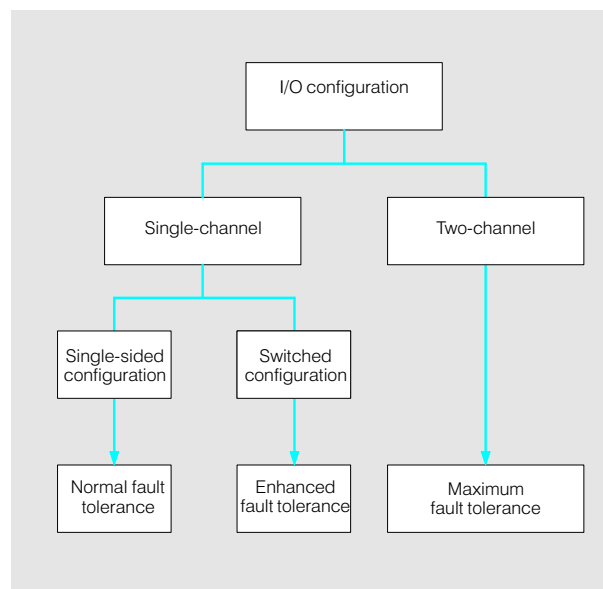
Fig. 3/8 Degrees of fault tolerance of the I/O area
