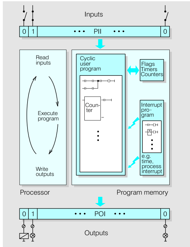
Fig. 3/4 Principle of operation of the S5-115U
