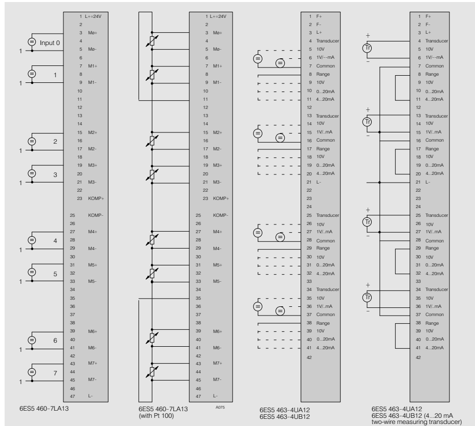
Fig. 3/30 Connection diagram for analog input modules
