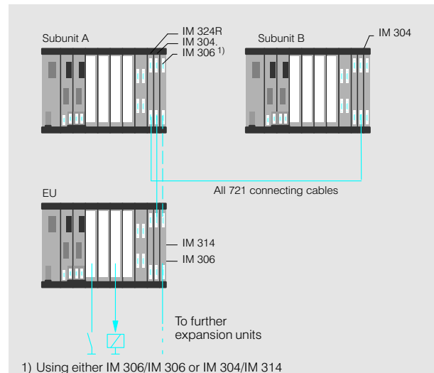
Fig. 3/9 Single-sided configuration (normal fault tolerance)
