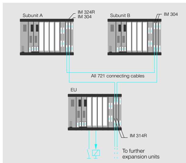
Fig. 3/10 Switched configuration (enhanced fault tolerance)
