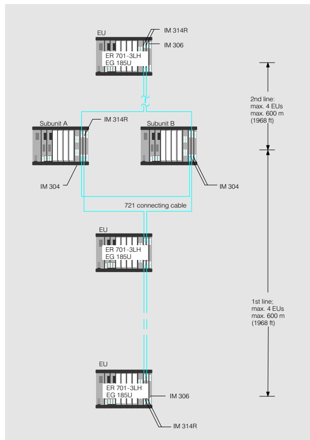
Fig. 3/39 Distributed switched configuration of I/O modules
