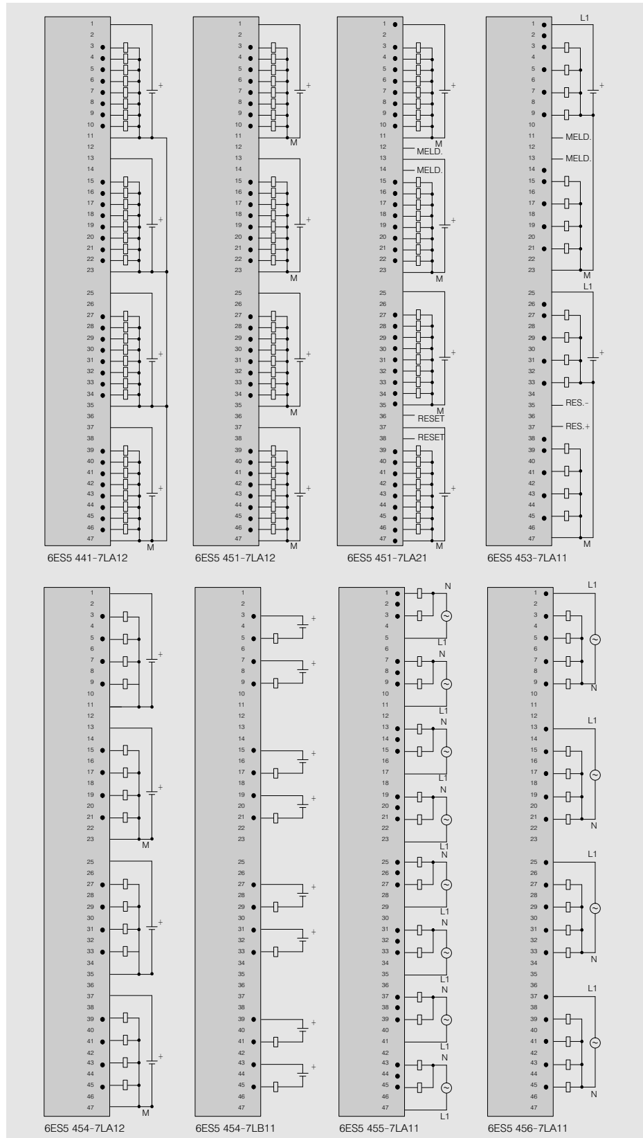
Fig. 3/27 Connection diagrams for digital output modules
