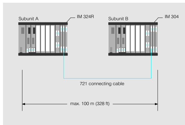
Fig. 3/38 Interfacing of central controllers
