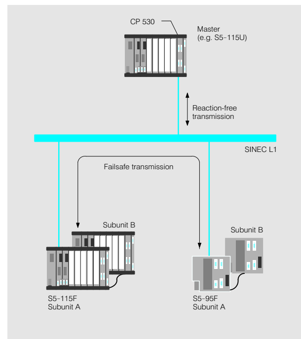
Fig. 3/23 Single-channel, safety-oriented link
