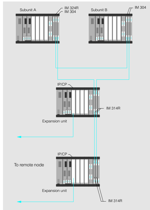
Fig. 3/13 IP/CP in switched redundant configuration
