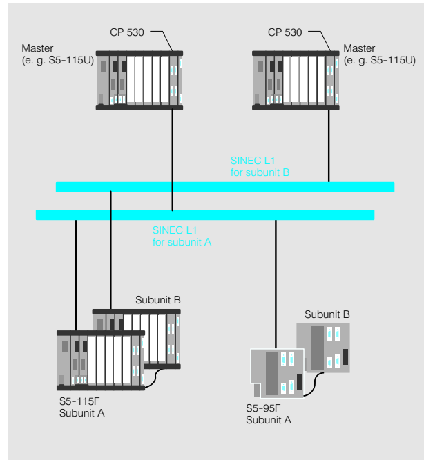
Fig. 3/24 Two-channel, safety-related link
