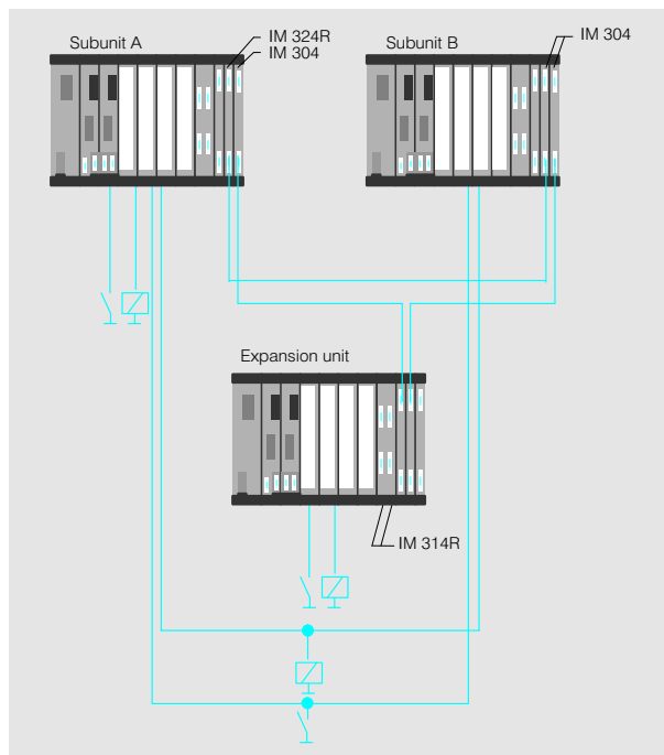
Fig. 3/12 Mixed configuration of an S5-115H
