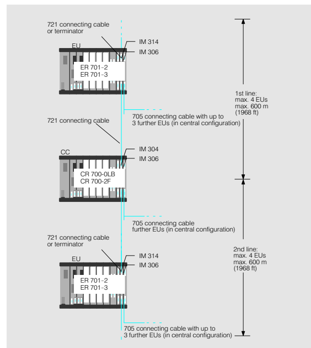
Fig. 3/42 Distributed configuration of expansion units
