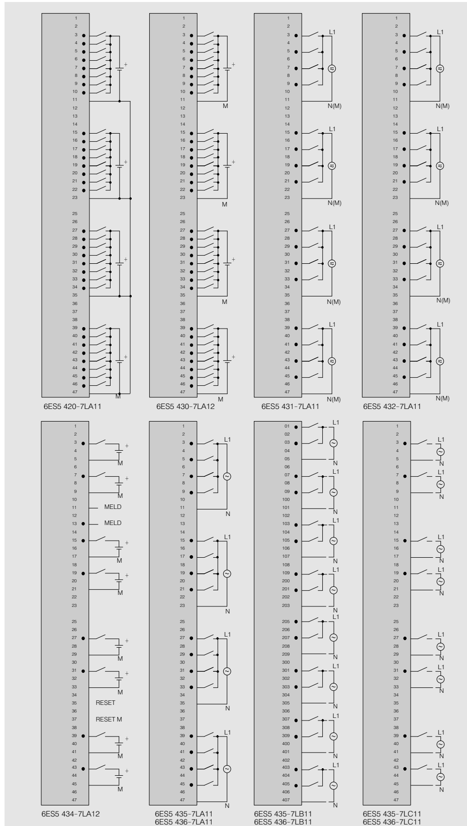
Fig. 3/25 Connection diagrams for digital input modules
