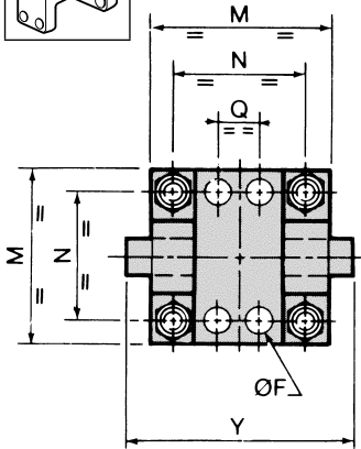
MOUNTING Complete trunnion mounting w/ angular clevis bracket CNOMO 06-07-11
