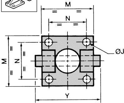
MOUNTING Complete trunnion mounting w/ angular clevis bracket CNOMO 06-07-11
