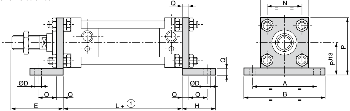
MOUNTING Foot, high and broad CNOMO 06-07-06
