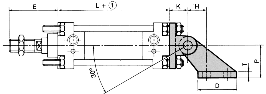
MOUNTING Complete trunnion mounting w/ angular clevis bracket CNOMO 06-07-11
