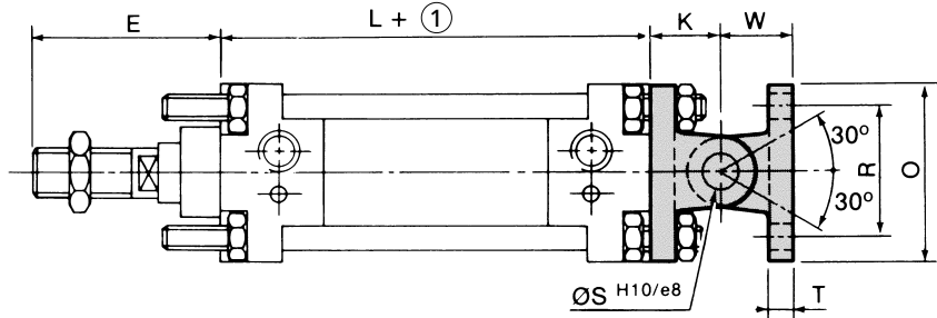
MOUNTING Complete trunnion mounting w/ angular clevis bracket CNOMO 06-07-11
