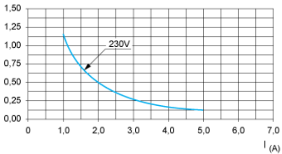
Courbes AC12
