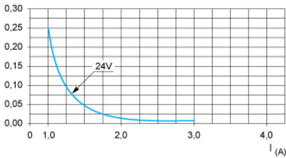
Courbes DC13
