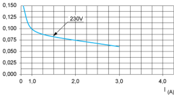
Courbes AC15
