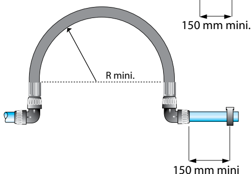
Expansion loop
