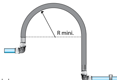
Obstacle bypass
