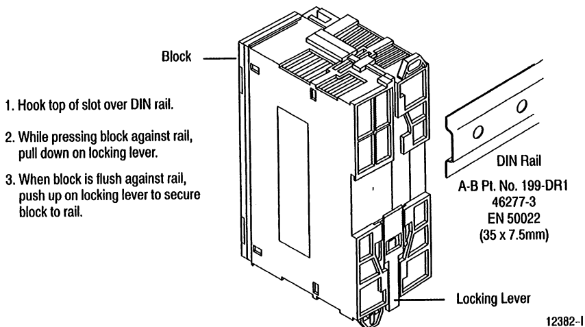
Figure 2 Mounting on a DIN Rail
