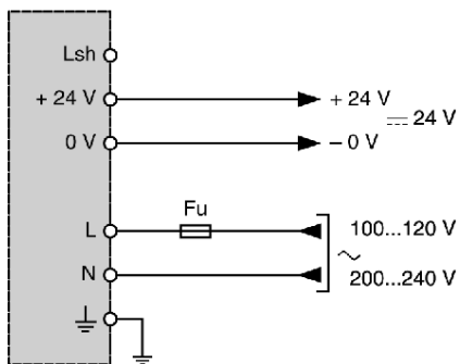
Raccordement normal
