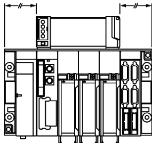
Racks 6 positions (TSX RKY 6/6EX)
