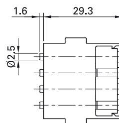
Pin side
