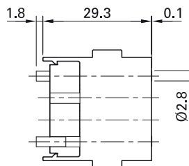
Socket side
