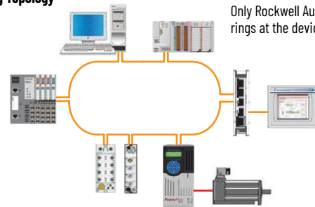
Ring Topology
