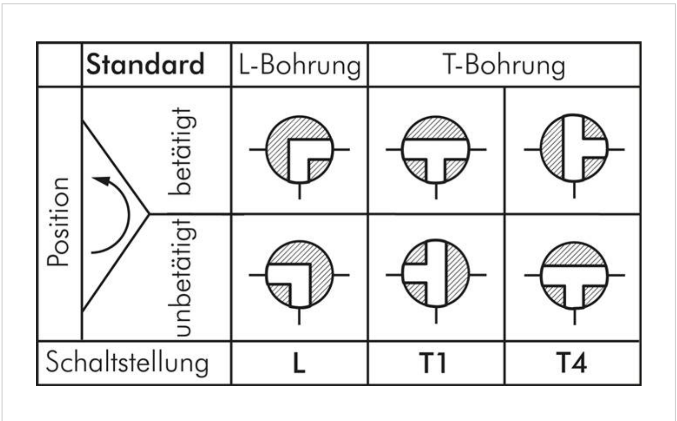
Drawing: Switching position
