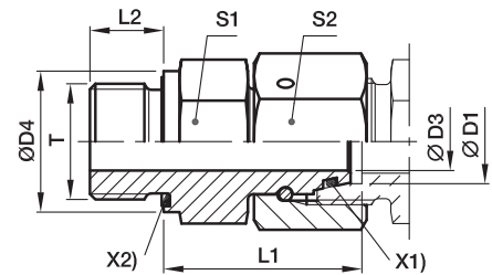
X2) Eolastic-sealing ED X1) O-ring OR
