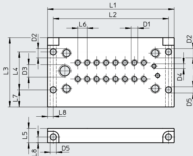
Pneumatic multiple connector plate with flange – CPV10/14/18
