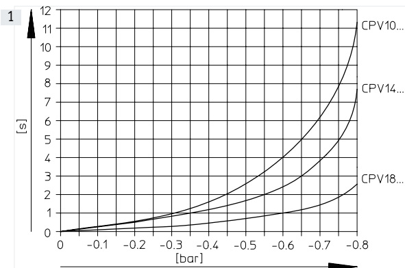
Evacuation time for a volume of 1 litre at P nom
