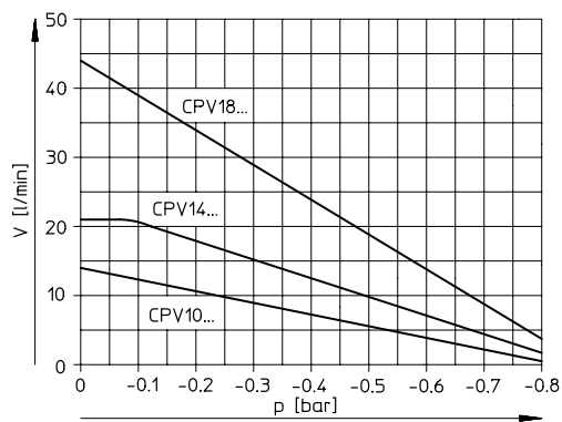
Suction capacity as a function of negative pressure at P nom
